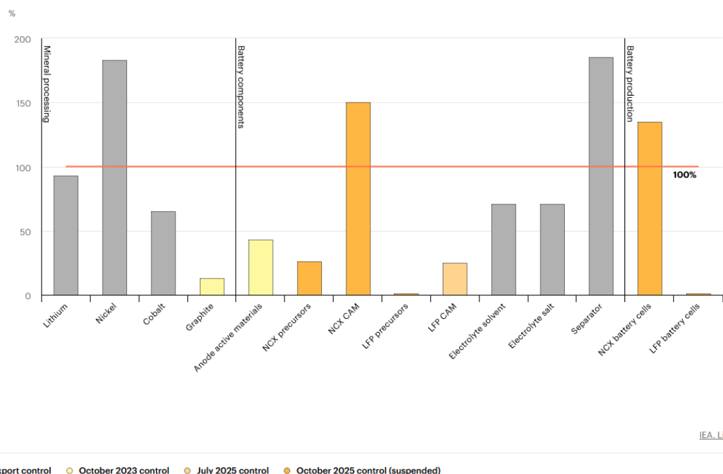
FIGURE 7 SHARE OF LITHIUM-ION BATTERY DEPLOYMENT OUTSIDE CHINA THAT COULD BE MET WITHOUT SUPPLY FROM CHINA, 2024; SOURCE: IEA. LICENCE CC BY 4.0
