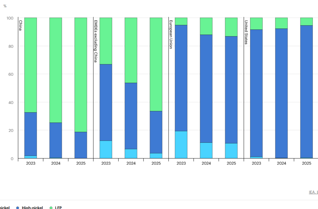
FIGURE 6 SHARE OF FOUR WHEELERS ELECTRIC VEHICLE BATTERY SALES BY CHEMISTRY AND REGION, 2023-2025; SOURCE: IEA. LICENCE CC BY 4.0
